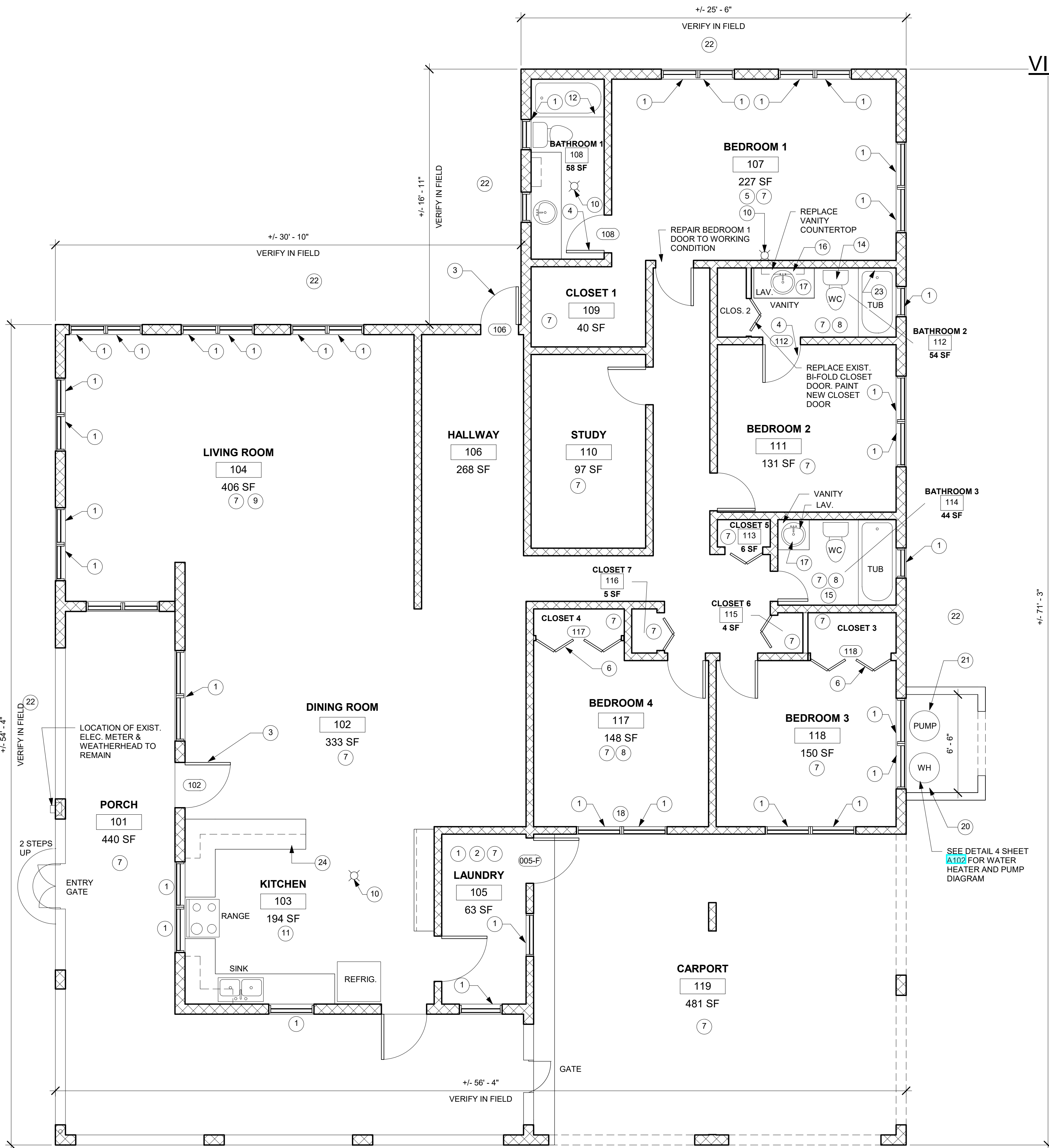
1 FIRST LEVEL FLOOR PLAN 1/4" = 1'-0"
