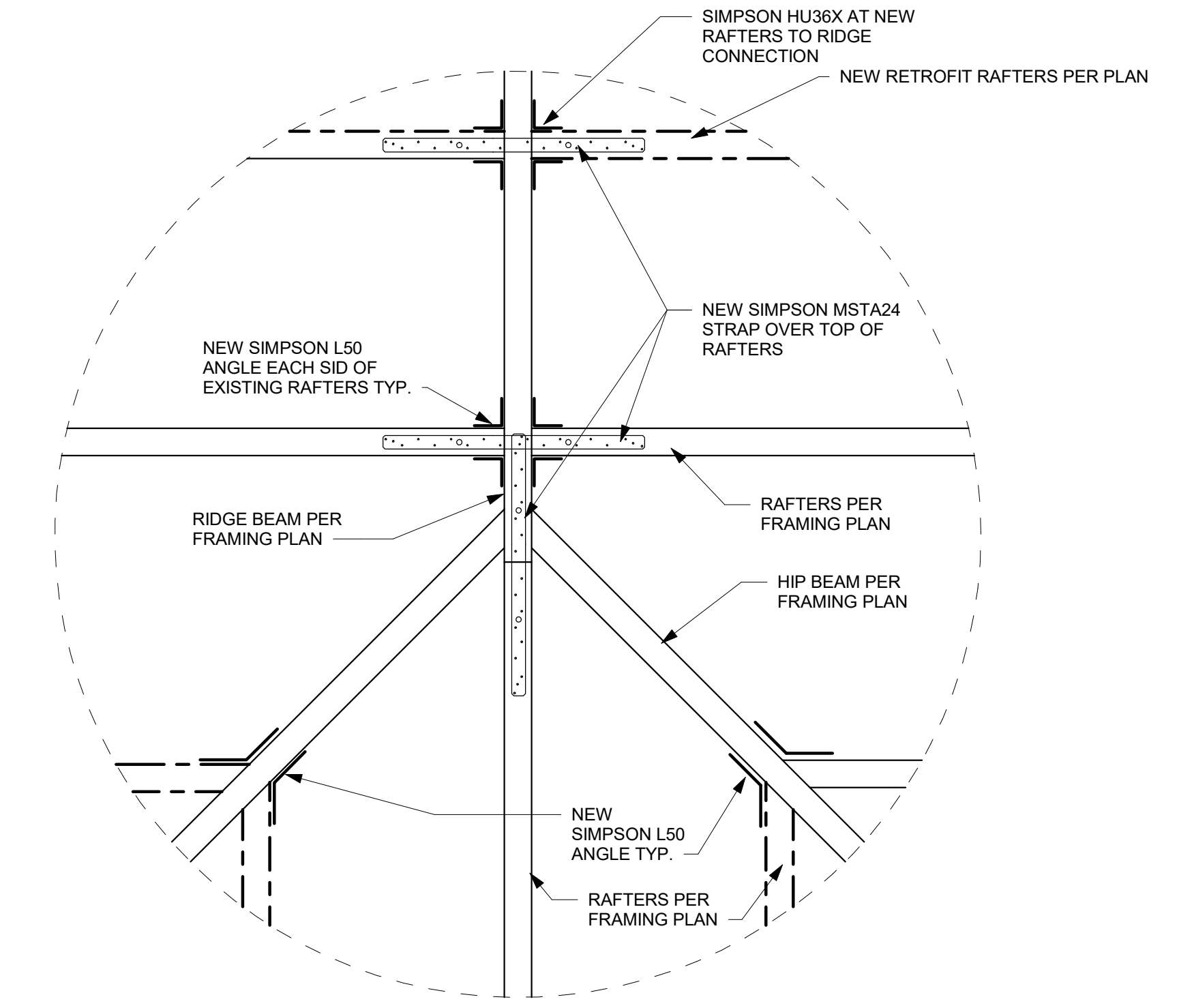
RIDGE RAFTER RETROFIT CONN. DTL (PLAN)1
