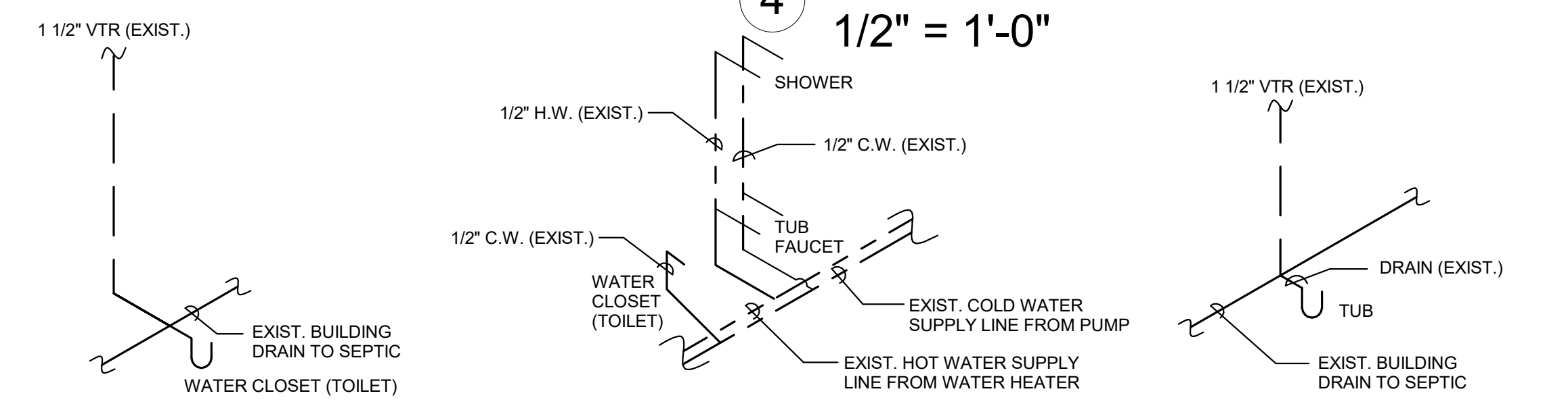
3 PLUMBING RISER DIAGRAMS 1/2" = 1'-0"
