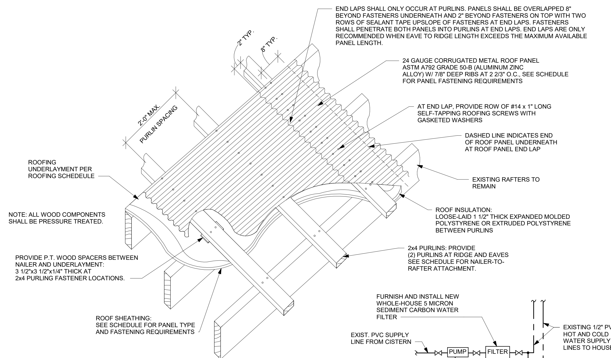
2 ROOF ASSEMBLY DETAIL 3/4" = 1'-0"
