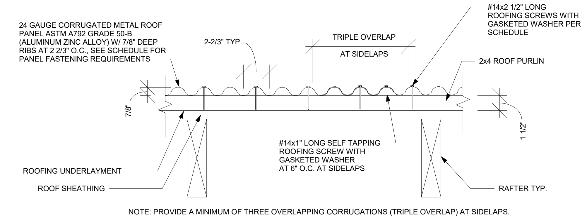
ROOF COVERING SECTION DETAIL
