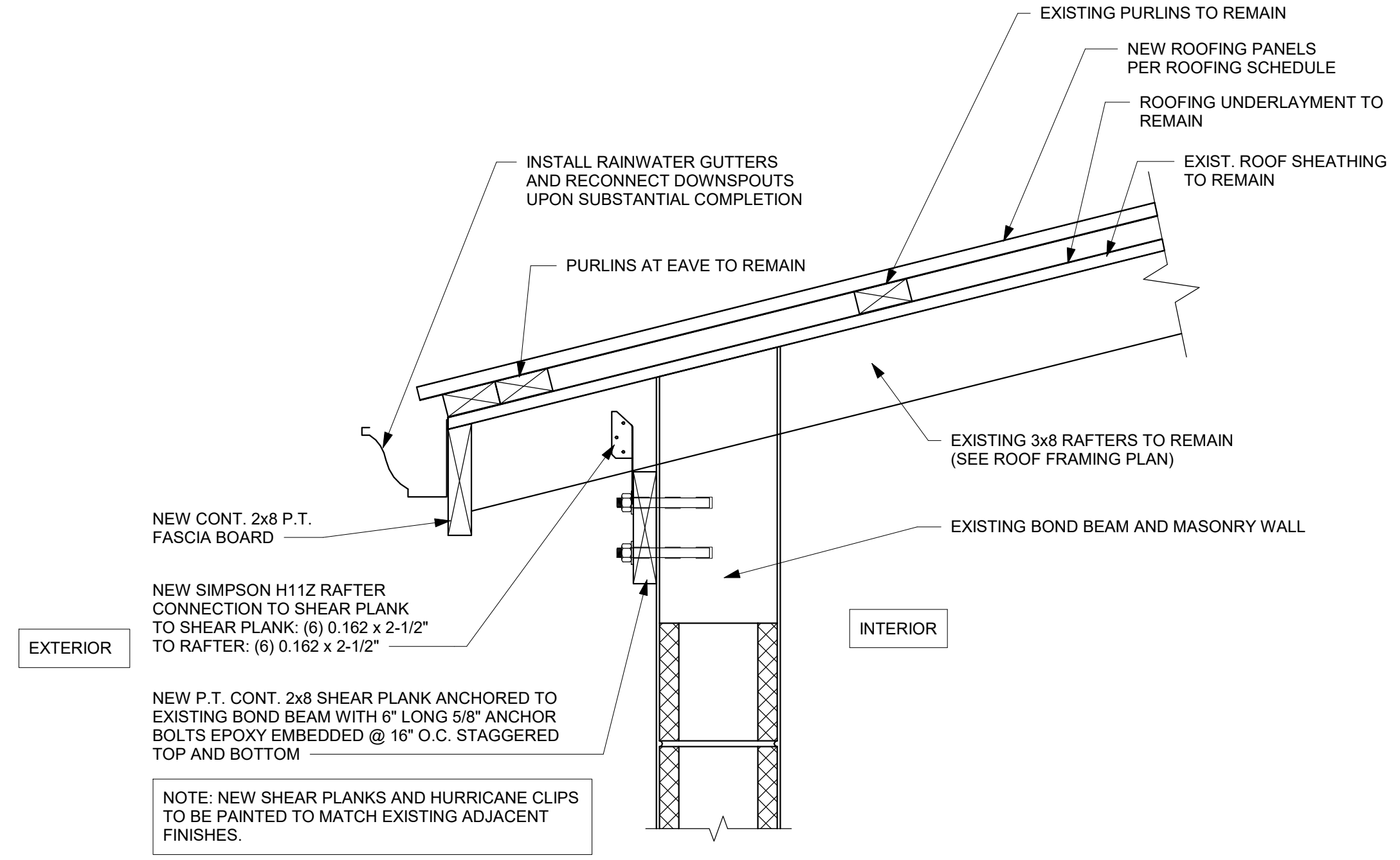
3 EAVE DETAIL - EXISTING RAFTER MITIGATION CONNECTION 1 1/2" = 1'-0"
