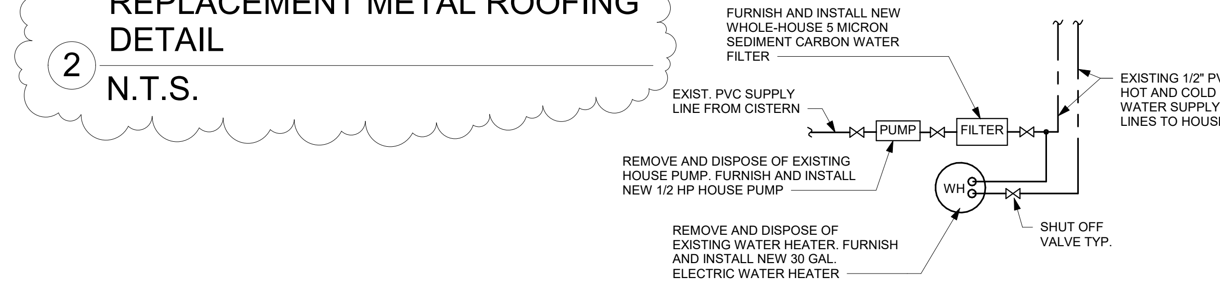
4 NEW WATER PUMP DIAGRAM N.T.S.
