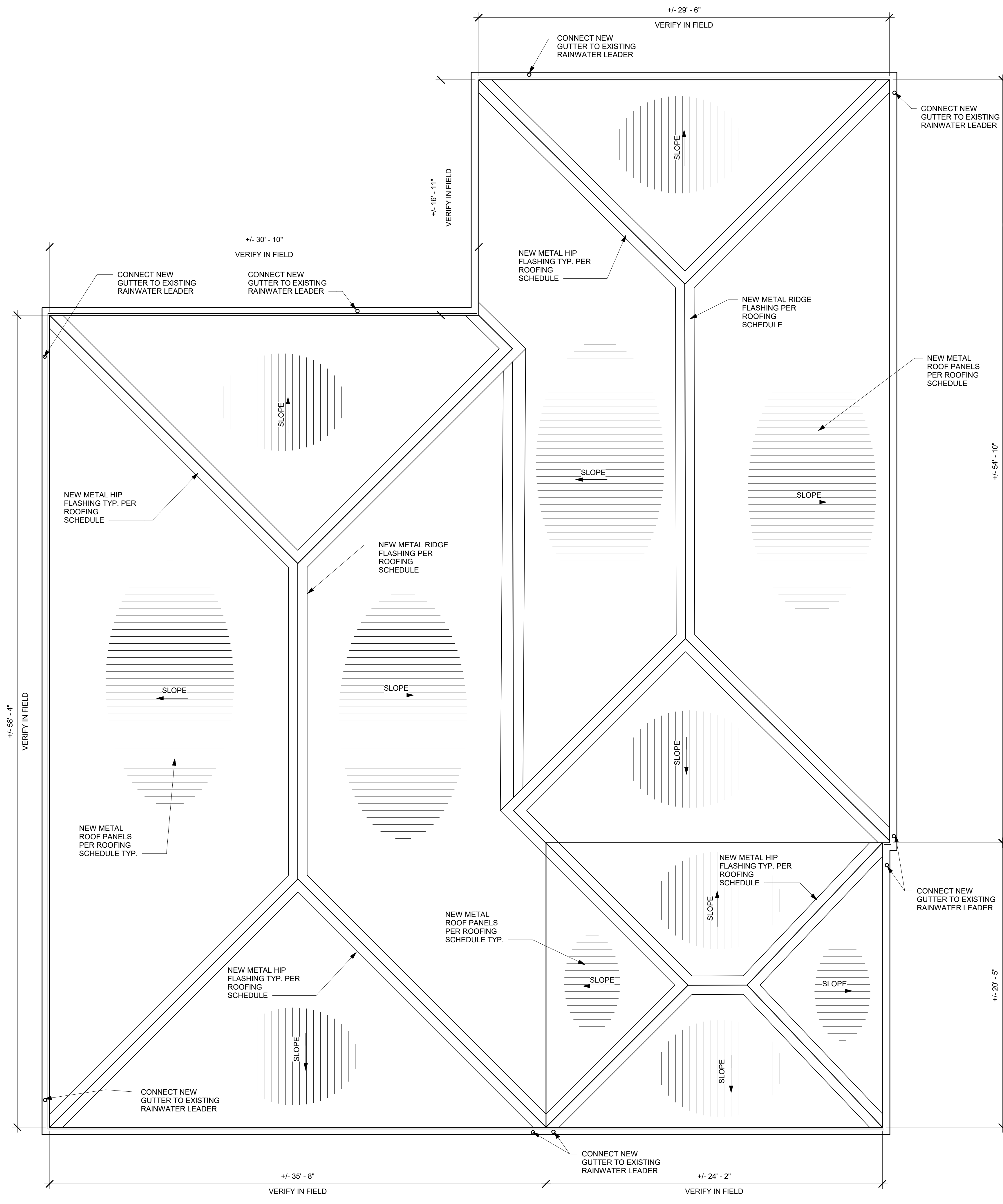
1 ROOF PLAN - NEW 1/4" = 1'-0"
