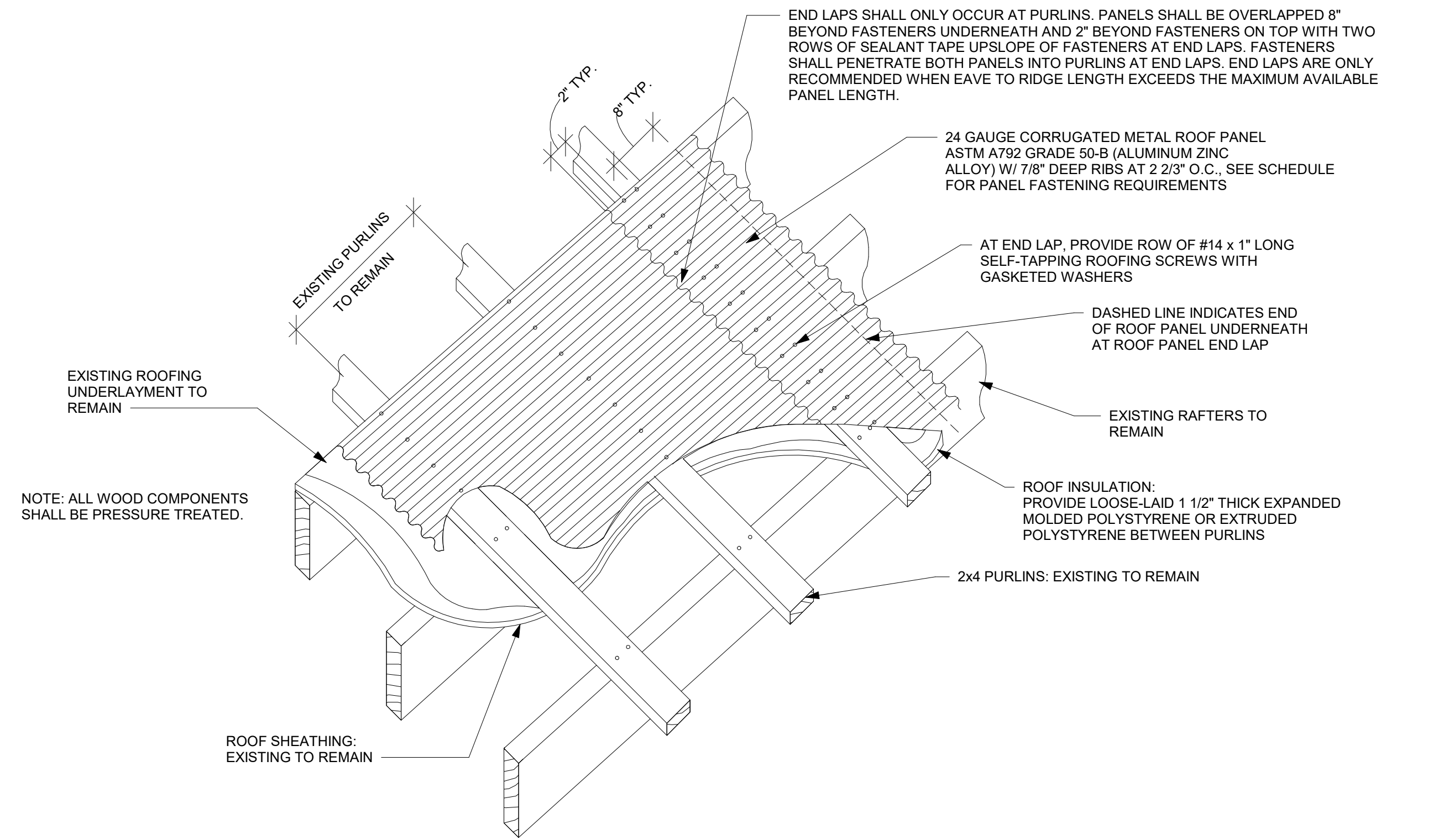
2 REPLACEMENT METAL ROOFING N.T.S.
