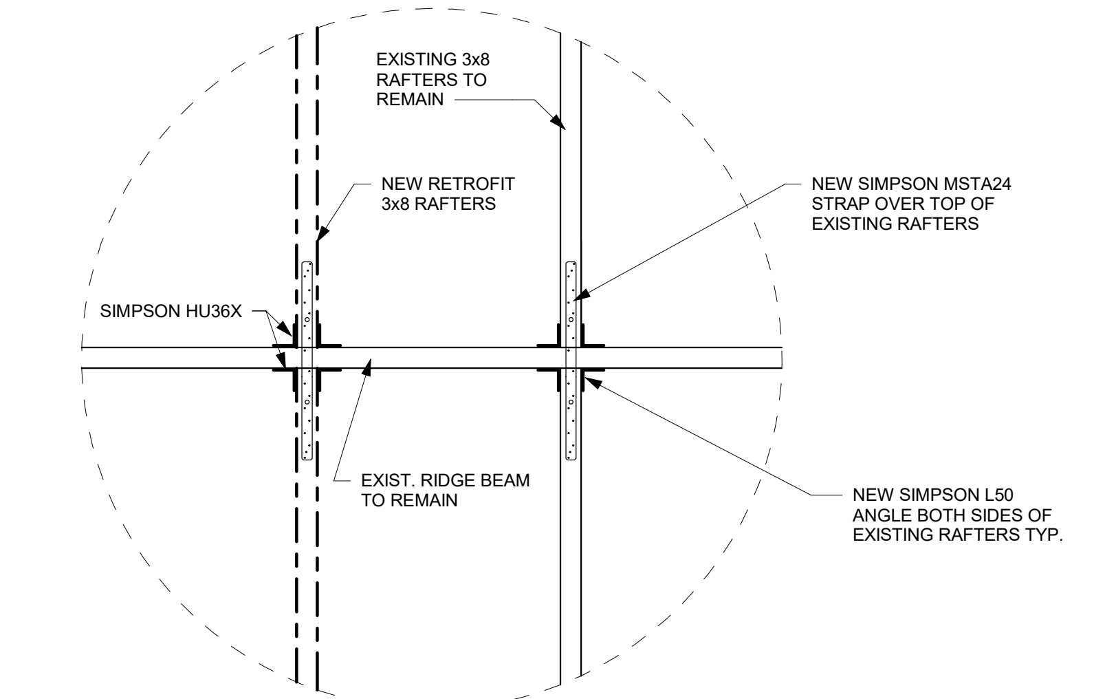
RIDGE RAFTER RETROFIT CONN. DTL (PLAN)
