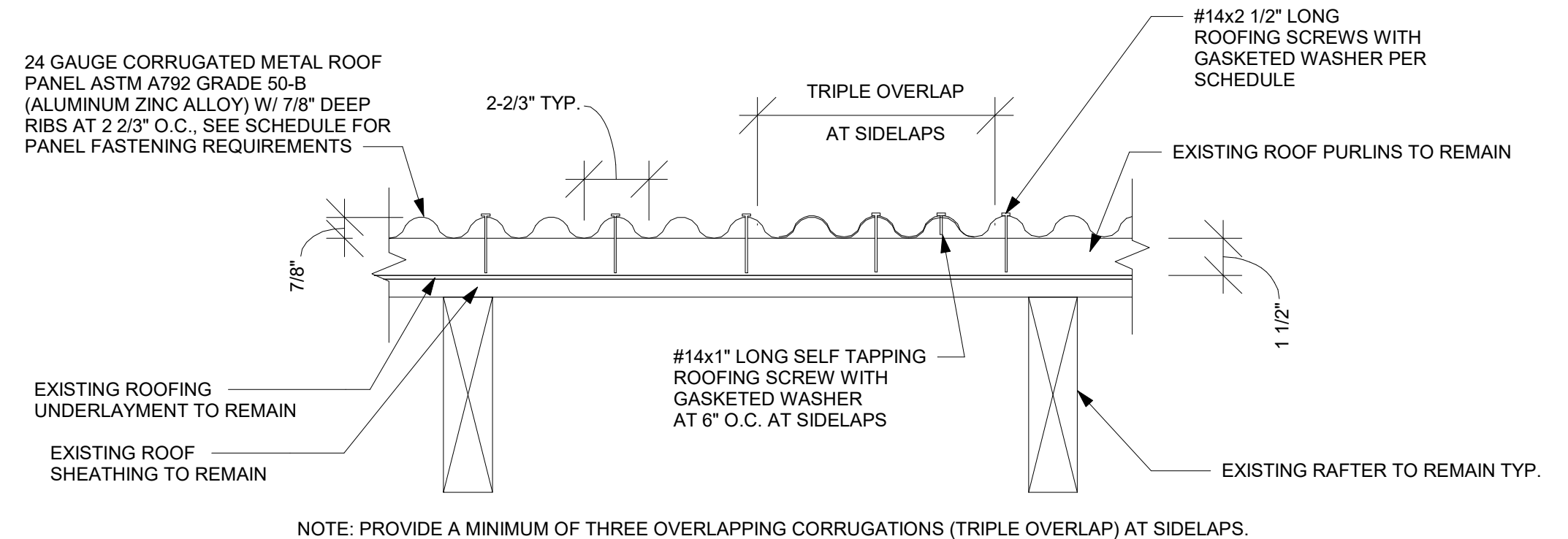
2 ROOF COVERING SECTION DETAIL 1" = 1'-0"
