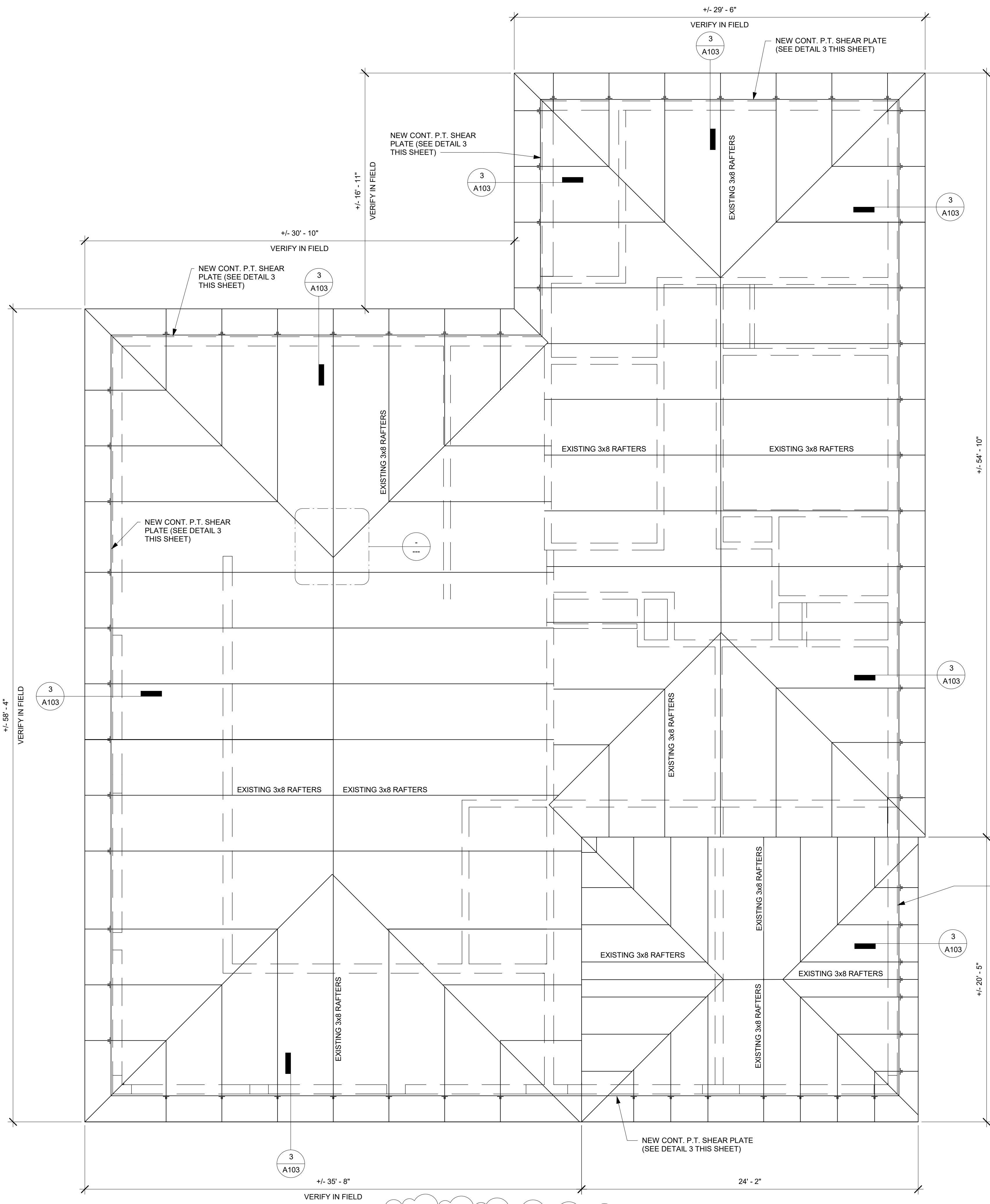
1 ROOF FRAMING PLAN 1/4" = 1'-0"
